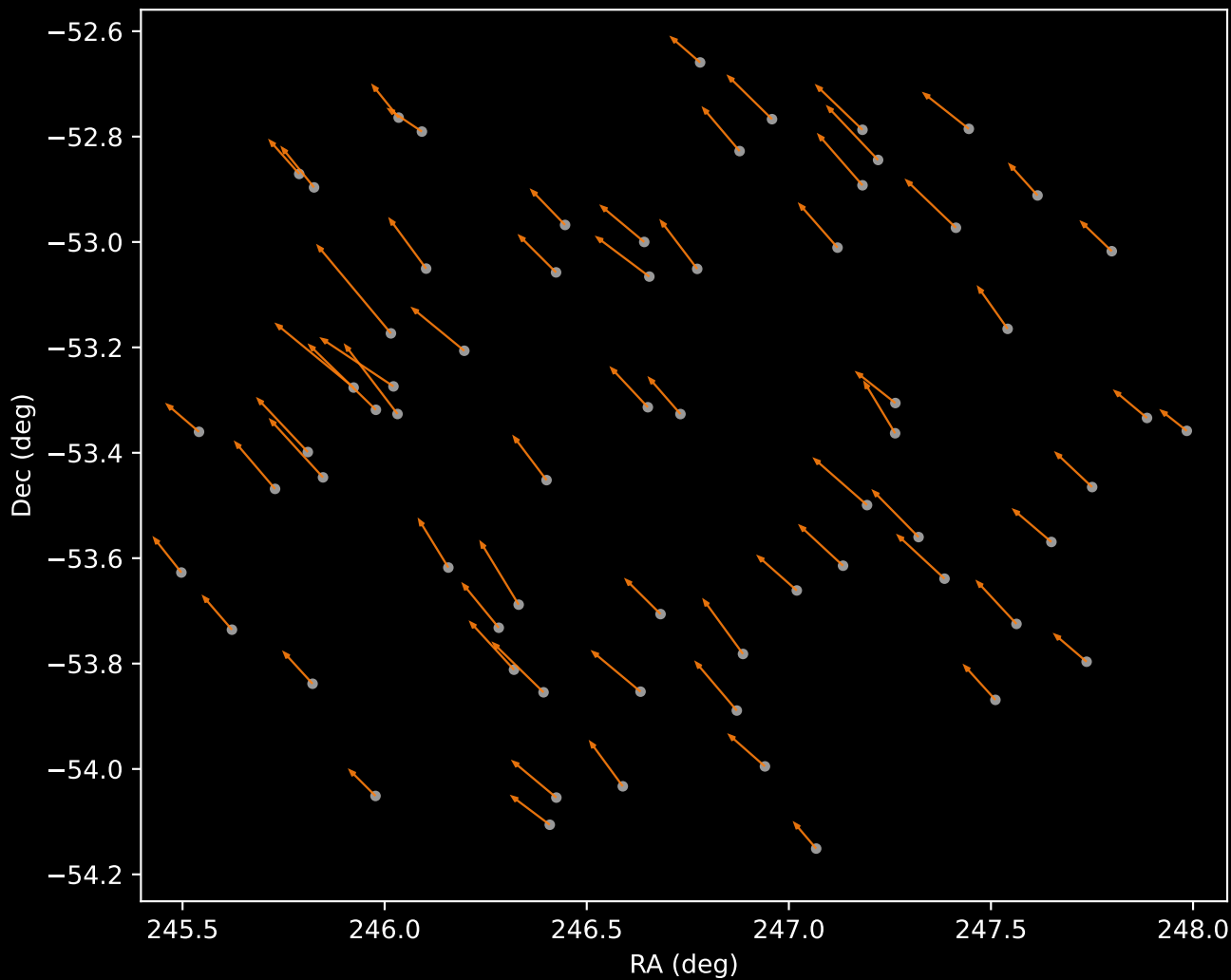
APOGEE DR17 Cluster 2 Proper Motion Vectors (n=67)
