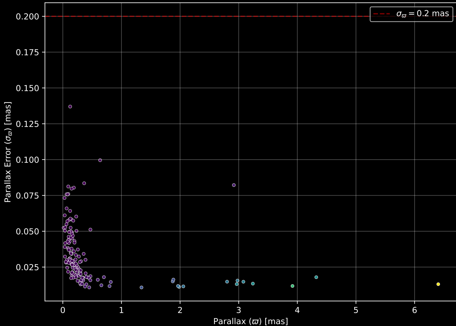
APOGEE DR17 Field: [278+00] Parallax Quality (n= 150)
