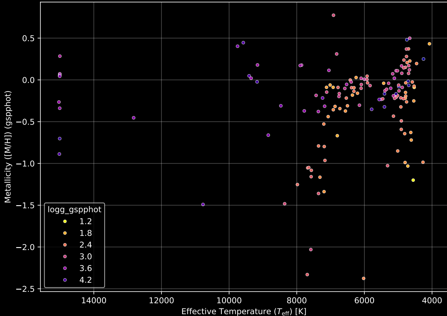
APOGEE DR17 Field: [278+00] Stellar Population Parameters (n= 150)
