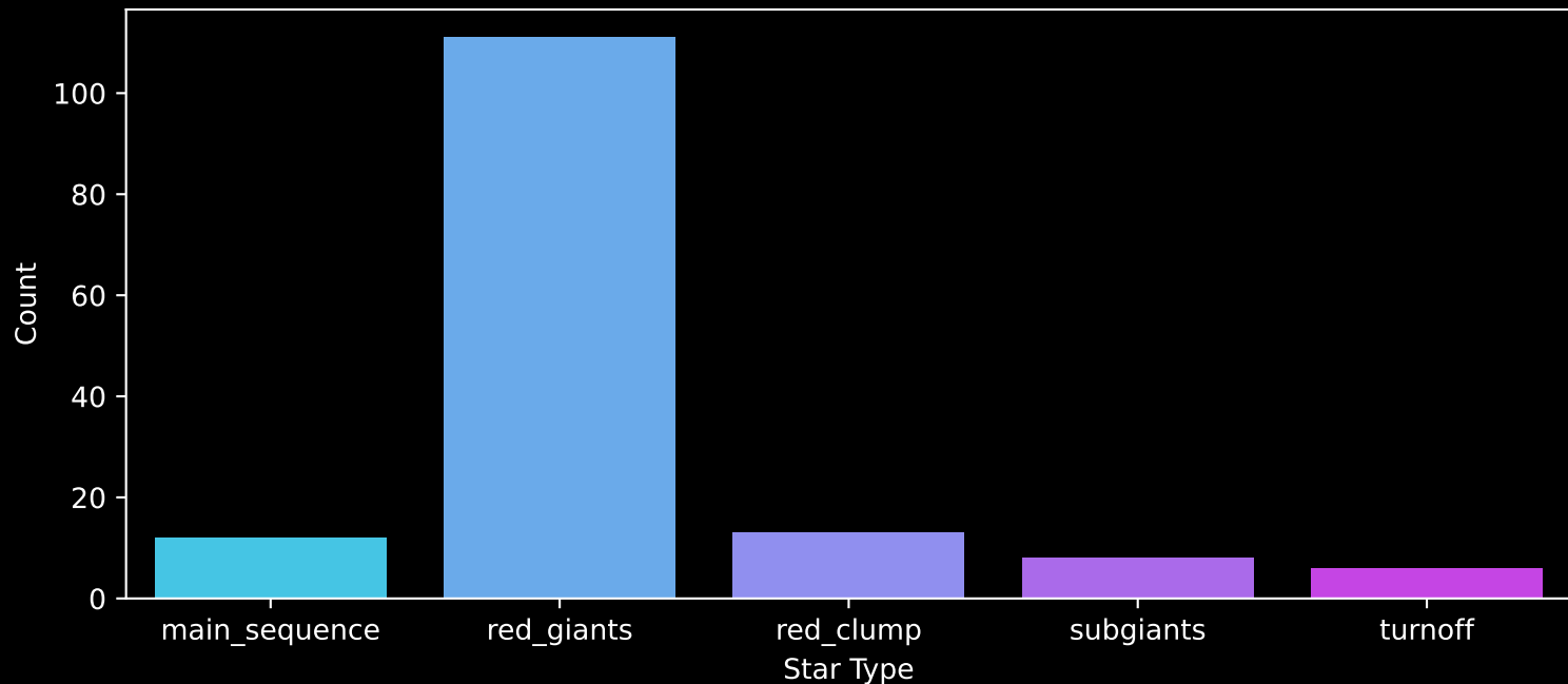
APOGEE DR17 Field: [278+00] Count plot of Star Type
