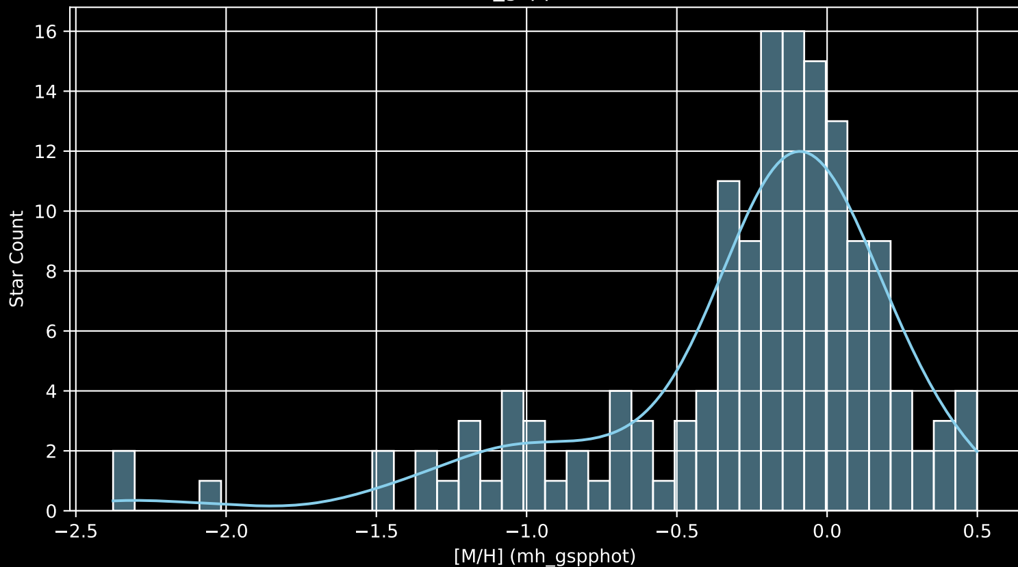
APOGEE DR17 Field: [278+00 [M/H] (mh_gspphot) (n= 149)
