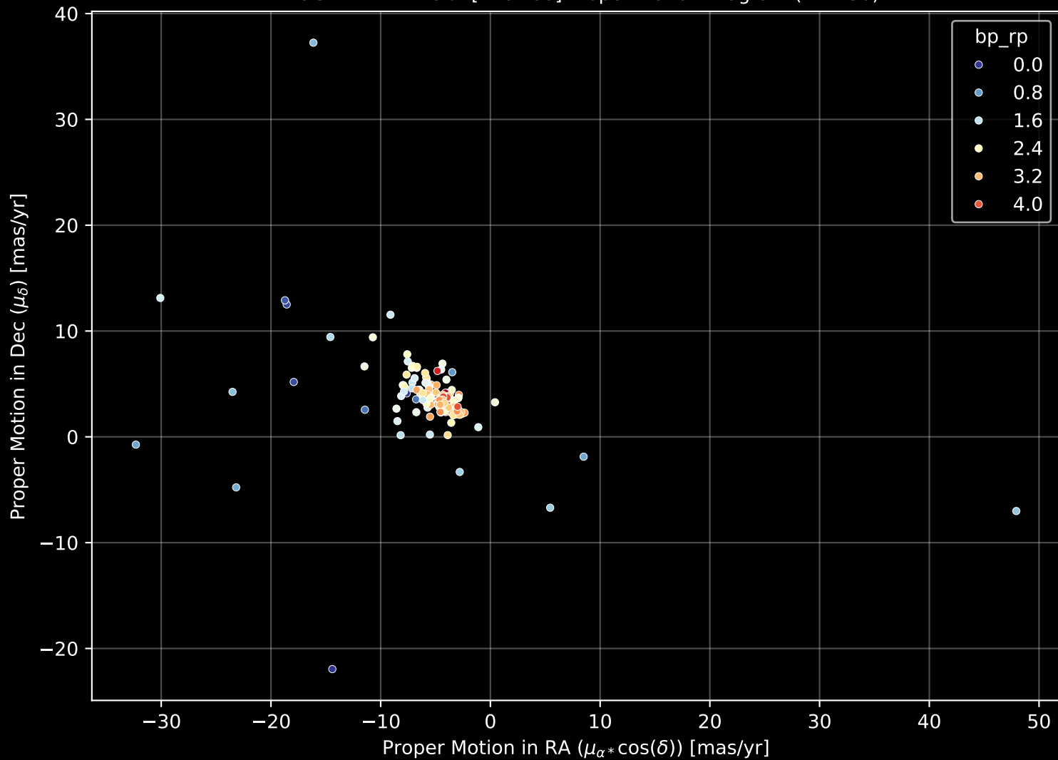
APOGEE DR17 Field: [278+00] Proper Motion Diagram (n= 150)
