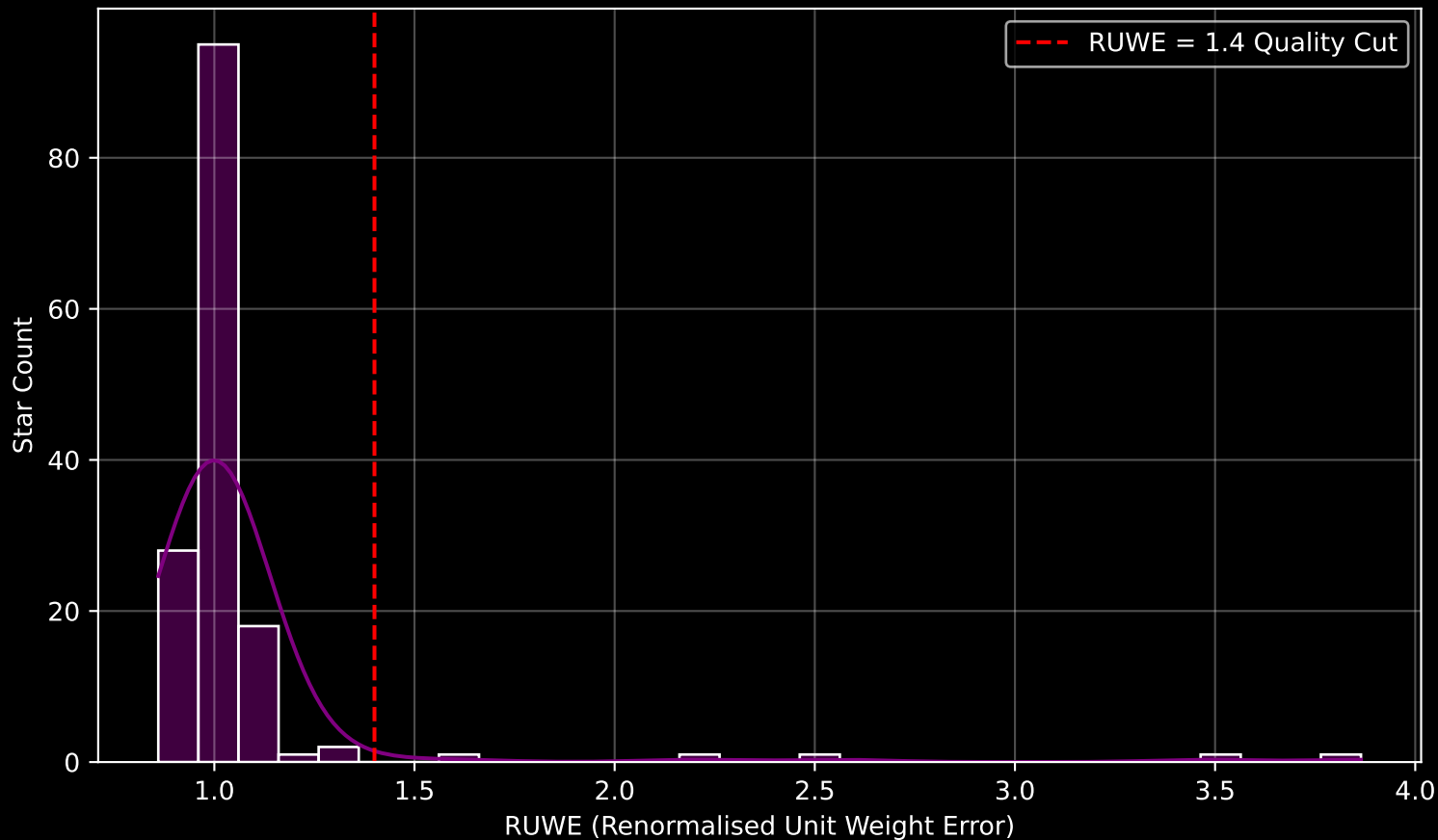
GAPOGEE DR17 Field [278+00] RUWE Distribution (n= 149)
